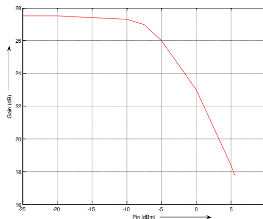
Fig 3: Gain of the Power amplifier
