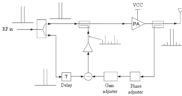
Figure 4: RF feedback linearization topology
