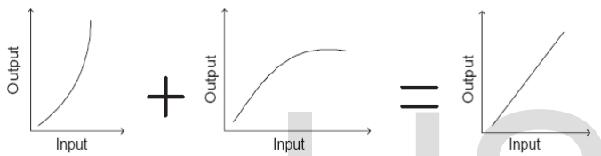
Figure 7: Basic steps of Predistortion
