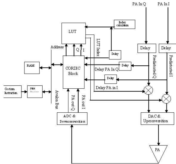
Fig 8: Proposed Digital Predistortion system
