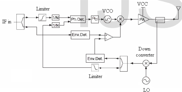
Figure 5: Polar loop linearization topology
