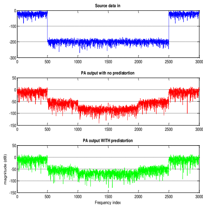
Fig 10: Normalized Linearity of Power amplifier
