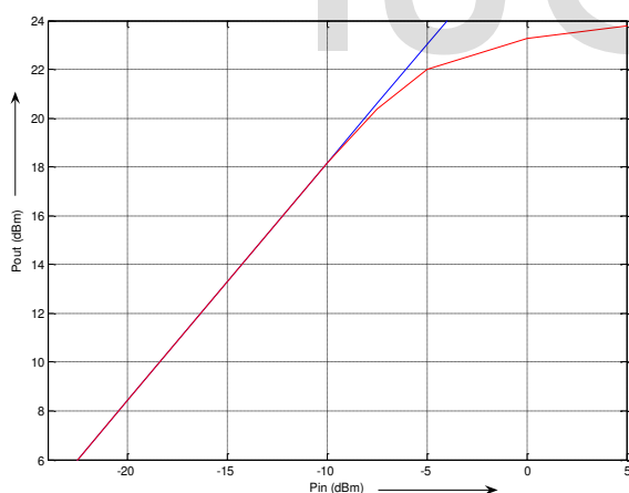
Fig 2. Output power characteristics of power amplifier
